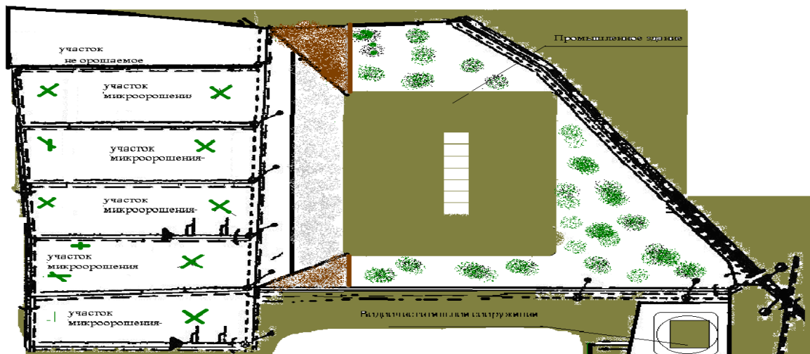
Fig.2. Scheme of the irrigation sprinkling station on the experimental part of the Tertersky RWCN in the Garabagh land in the period 2006-2010 with the use of the Idad and MDR sprinklers:
