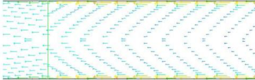
Fig. 7 Velocity vectors inside the pulse tube
