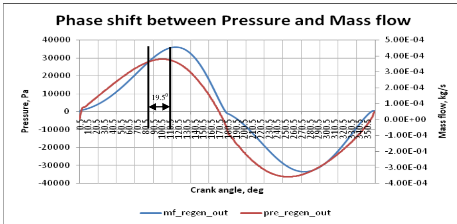
Fig. 5 Phase shift between peak pressure and mass flow at cold end for Orifice PTC
