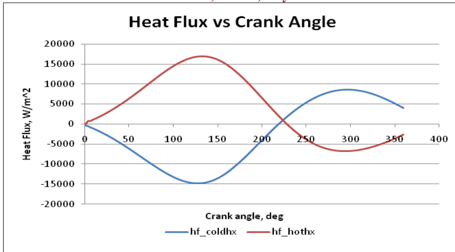
Fig. 4 Heat flux vs Crank angle at cold end for basic PTC
