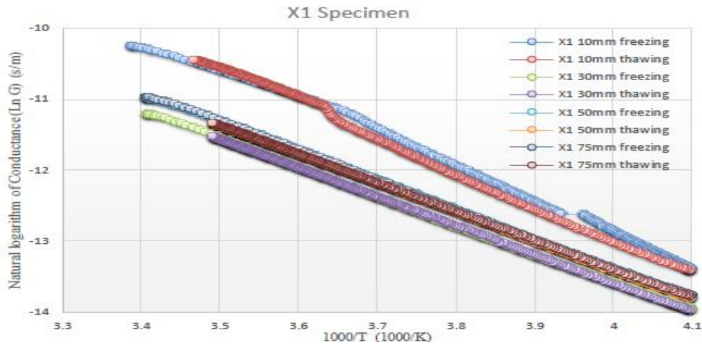
Fig 6: Natural logarithm of conductance vs 1000/T for specimen X1
