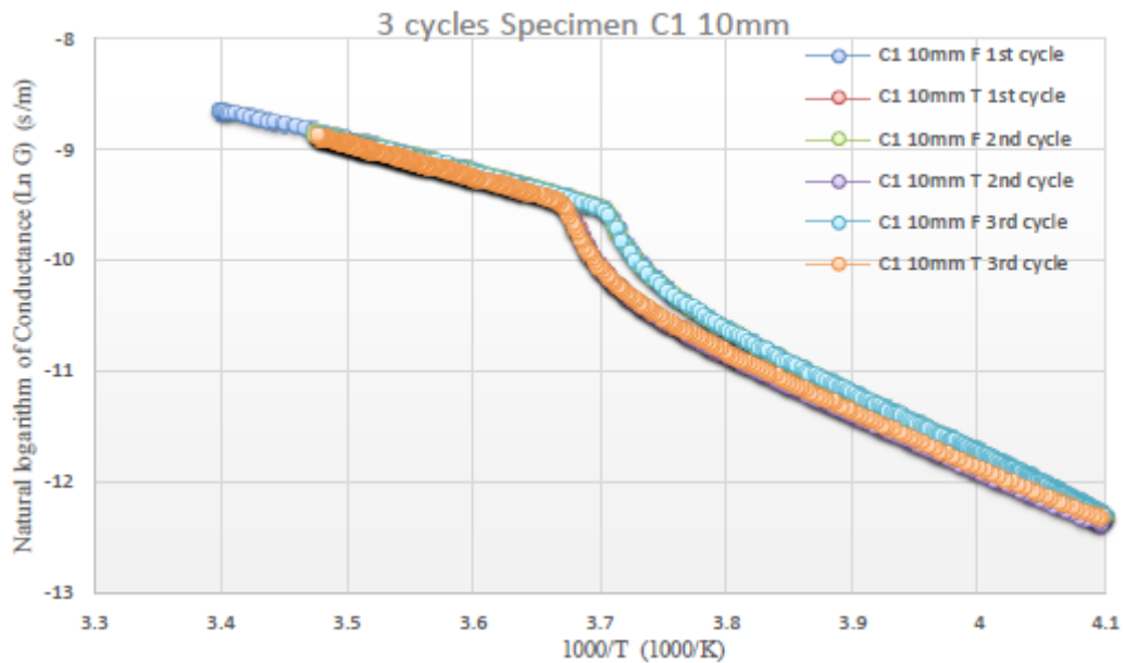
Fig 8: Natural logarithm of conductance vs 1000/T for specimen C110mm 3 cycles subjected to 3 cycles of freezing and thawing
