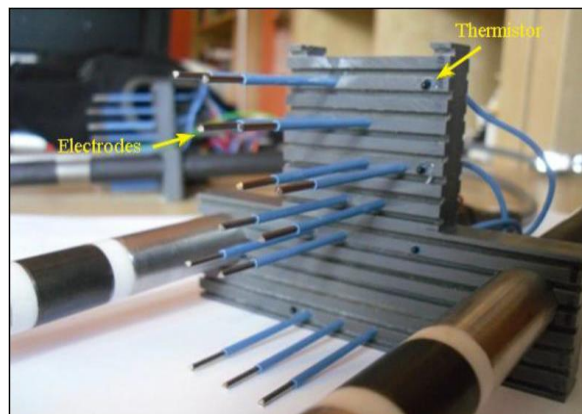
Fig 1: Multi Electrode sensor array
