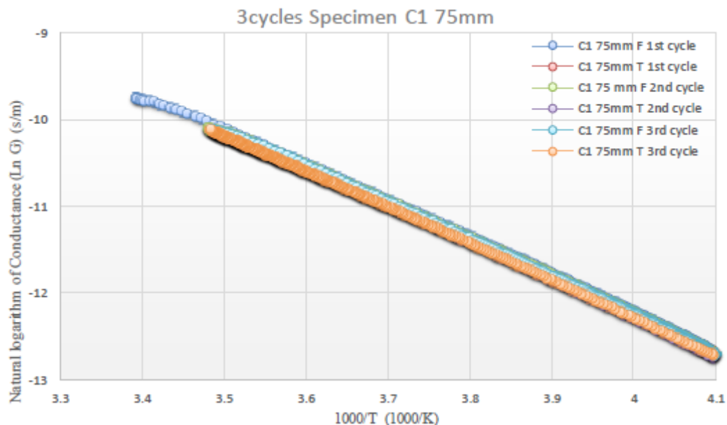
Fig 9: Natural logarithm of conductance vs 1000/T for specimen C1 75mm subjected to 3 cycles of freezing and thawing
