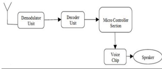
b)A design prototypic architecture for receiver unit
