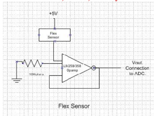
c) Flex sensor connected to LM258/LM358 op- amps
