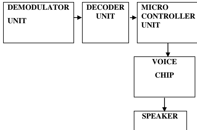
b)A design prototypic architecture for receiver unit
