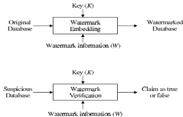
Fig 1. Watermarking Phases
