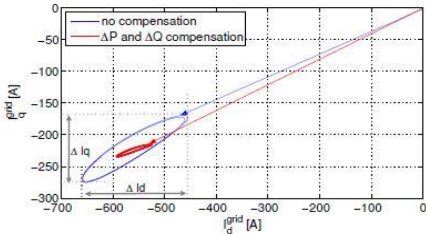
Fig. 10. Behaviour of the Power Grid Current Vector Within Dq0 Reference Frame
