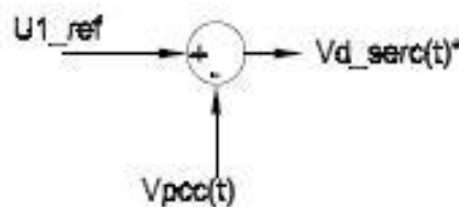
Fig. 5. Series Compensator Controller
