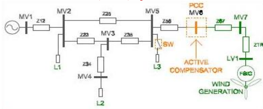
Fig 1. Study Case Power System
