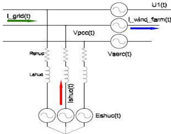
Fig. 4. Power Stage Compensator Model. AC Side
