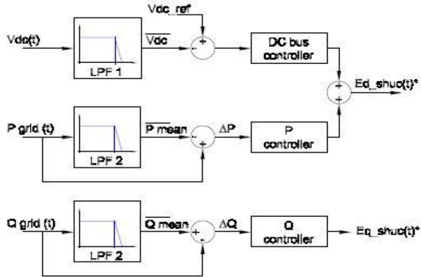
Fig 6 Shunt Compensator Controller
