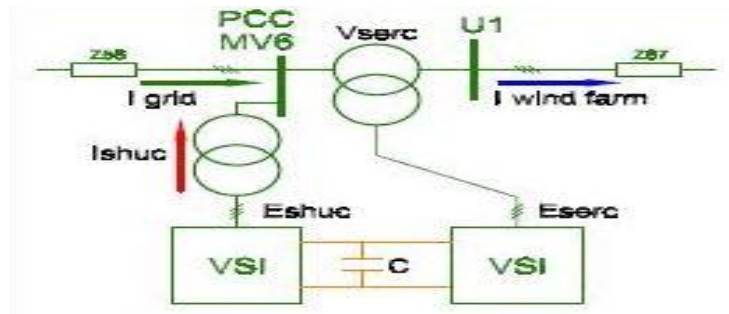
Fig 2 Block Diagram of UPQC
