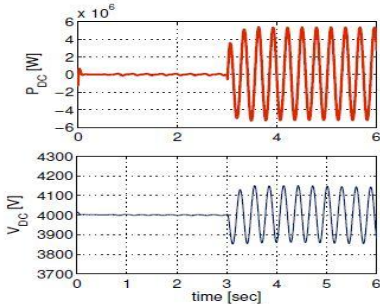
Fig. 9. Power and Voltage of the Capacitor in the DC-Bus.
