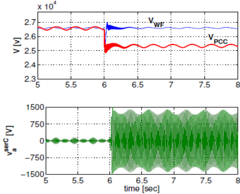
Fig. 11. Voltage at WF, at PCC, and Series Injected Voltage at "A" Phase
