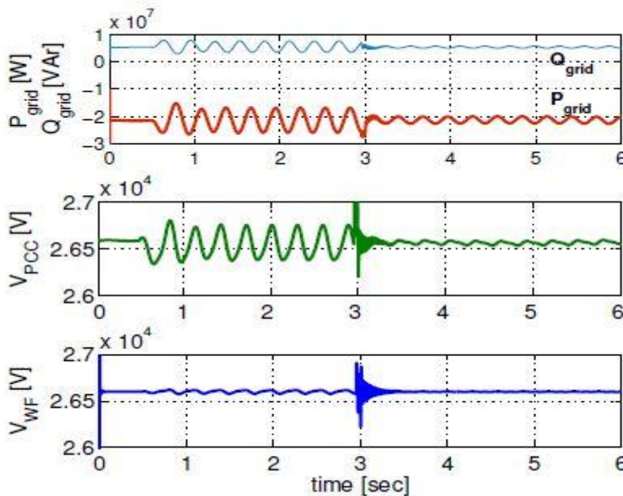
Fig. 8. Upper Curve: Active and Reactive Power Demand at Power Grid Side. Middle Curve: PCC Voltage. Lower Curve: WF Terminal Voltages
