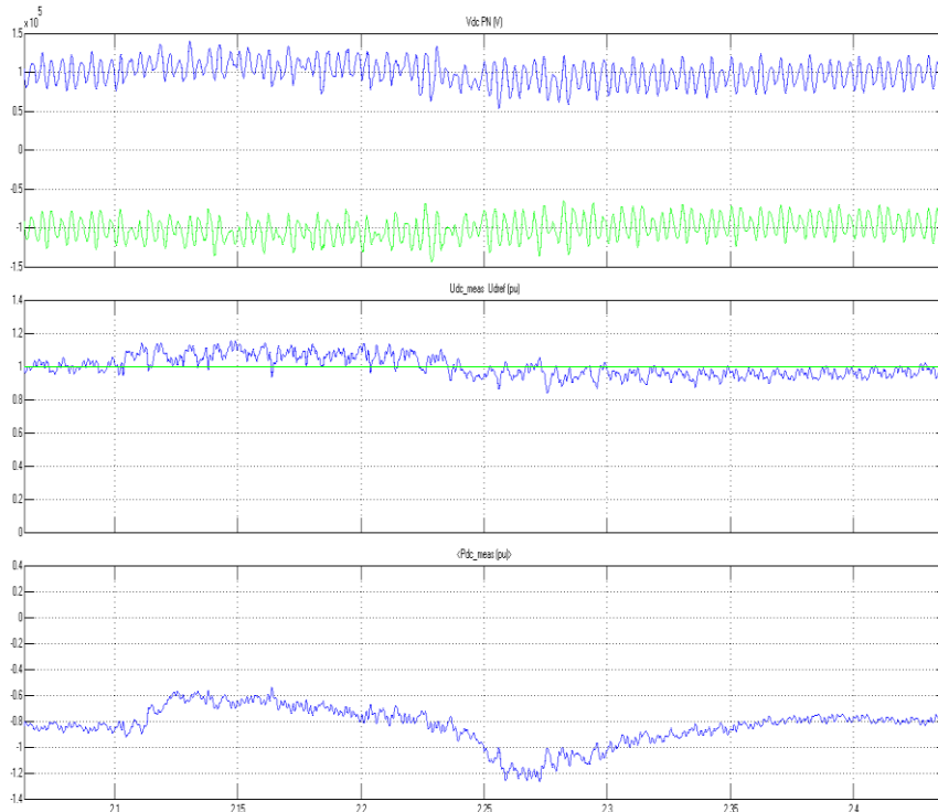
Fig 6 VSC HVDC transmission system During LG fault on the AC side of the inverter (a) DC line Voltage – Positive & Negative; (b) mean DC line voltage; (c) DC power transmitted
