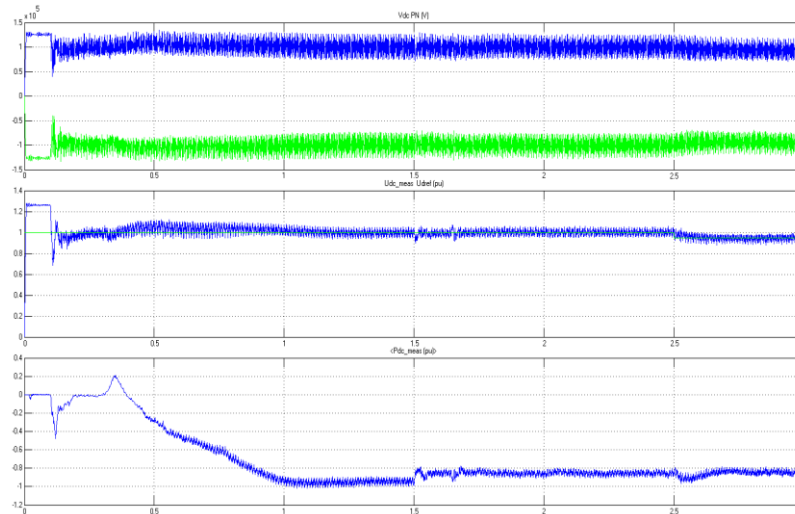
Fig 4. VSC HVDC transmission system without fault condition (a) DC line Voltage; (b) mean DC line voltage; (c) DC power transmitted
