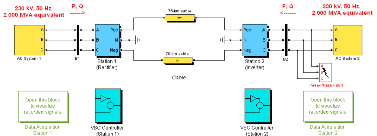
Fig.2. VSC-HVDC Transmission System Model
