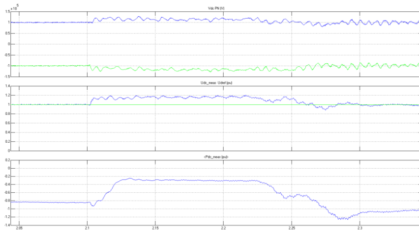
Fig 9 VSC HVDC transmission system During LLG fault on the AC side of the inverter (a) DC line Voltage – Positive & Negative; (b) mean DC line voltage; (c) DC power transmitted
