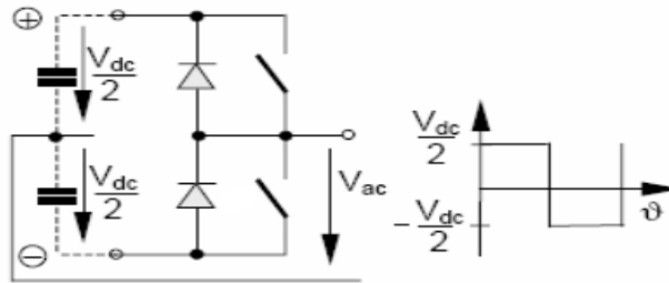
Fig 1. Operational principle of VSC
