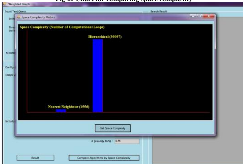
Fig 7:-Comparison of space complexity for a file.
