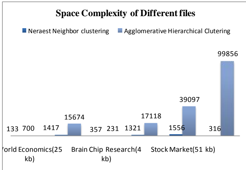
Fig 6:-Chart for comparing space complexity
