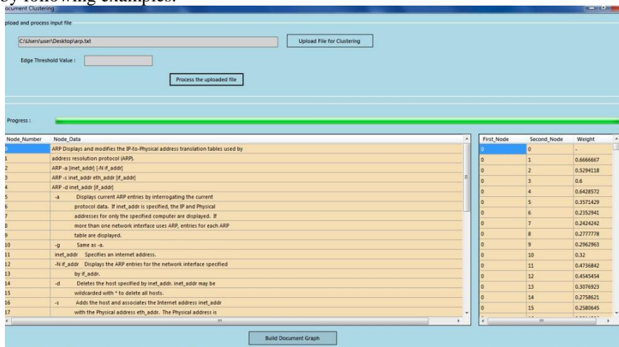
Fig 2:-Output screen of uploaded text file, processed file, document graph
