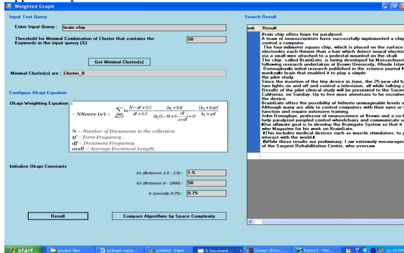
Fig 5:-Output screen of clustered summary result
