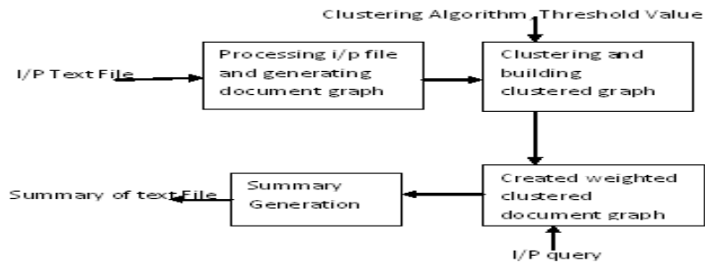
Fig 1 Architecture Diagram
