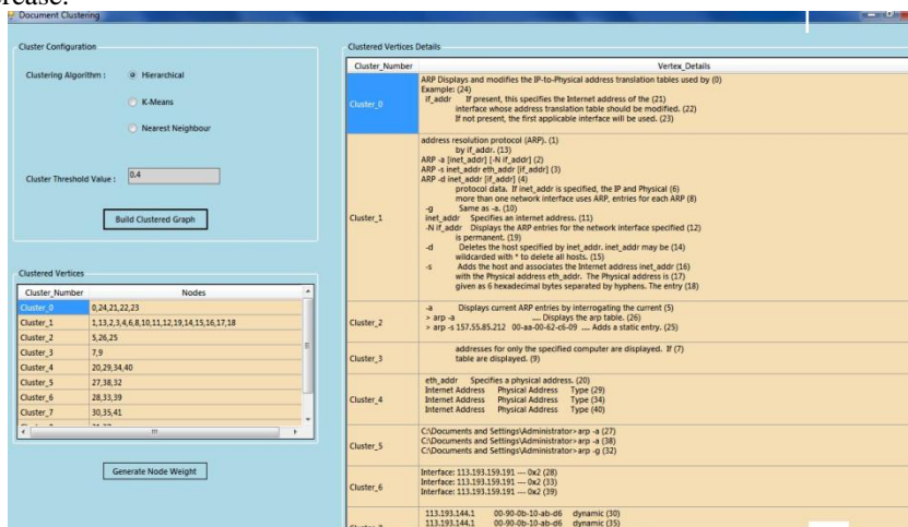
Fig 3:- Output screen of clustered document graph.
